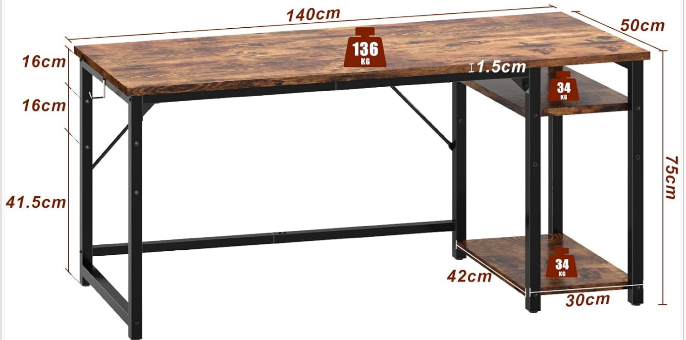
Figure 5: Detailed product dimensions for the JUMMICO desk, including shelf measurements.
