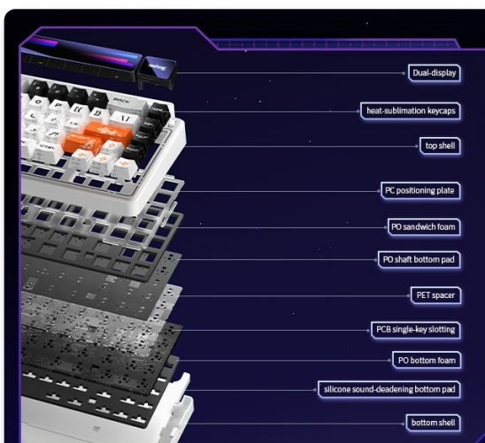
Figure 9: The advanced gasket structure for a soft and cushioned typing feel.
