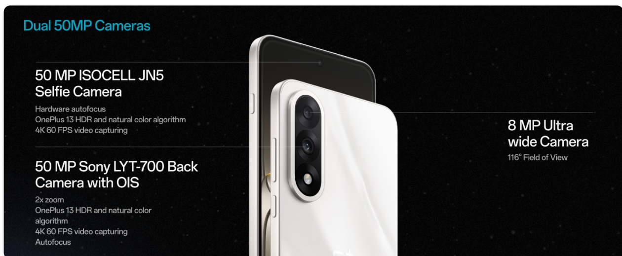
Image: Diagram showing the dual 50MP camera setup on the OnePlus Nord 5, detailing the specifications of the front and back sensors.
