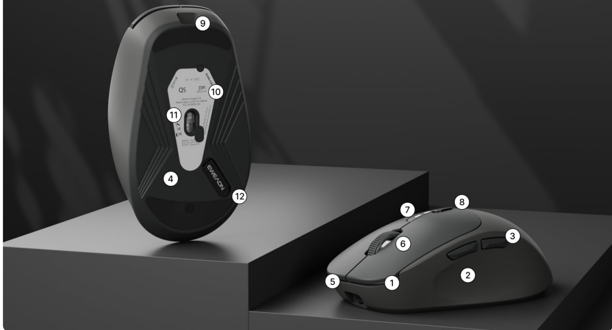
Figure 4: Labeled diagram of mouse components.
