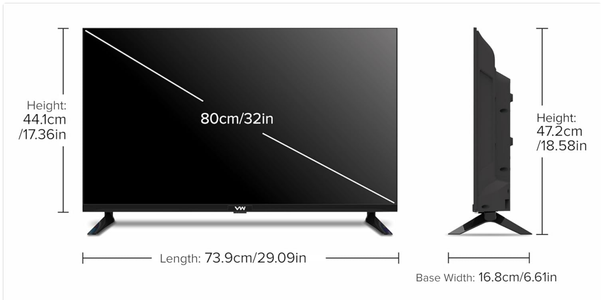
Figure 7.1: TV Dimensions.
