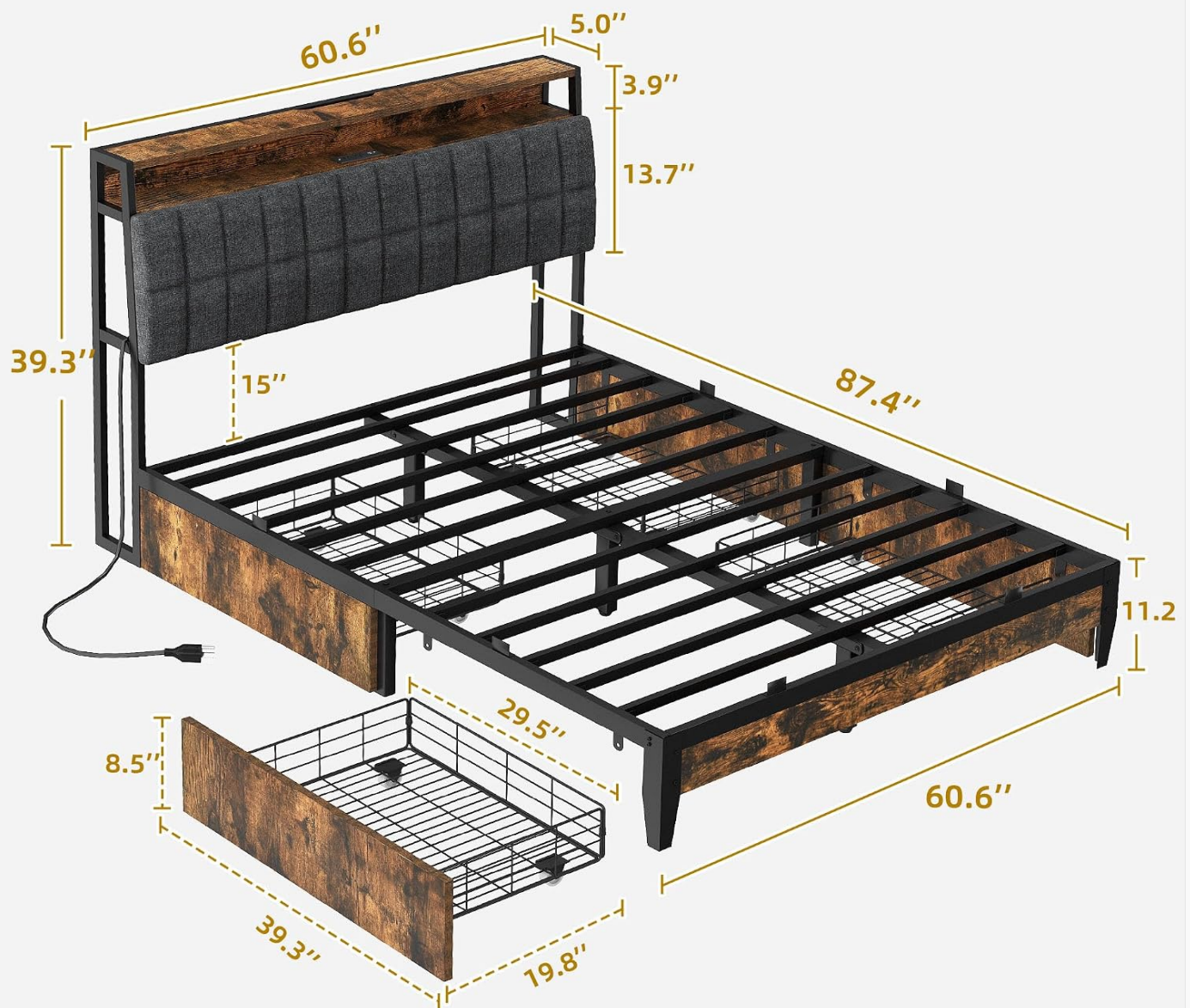
Image: Detailed dimensions of the YITAHOME Queen Size Platform Bed Frame, including height, width, length, and drawer measurements.
