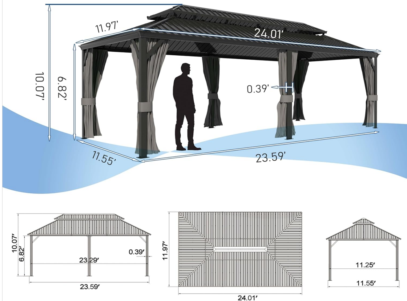
Figure 5: Detailed dimensions of the MUPATER 12X24 FT Hardtop Gazebo.
