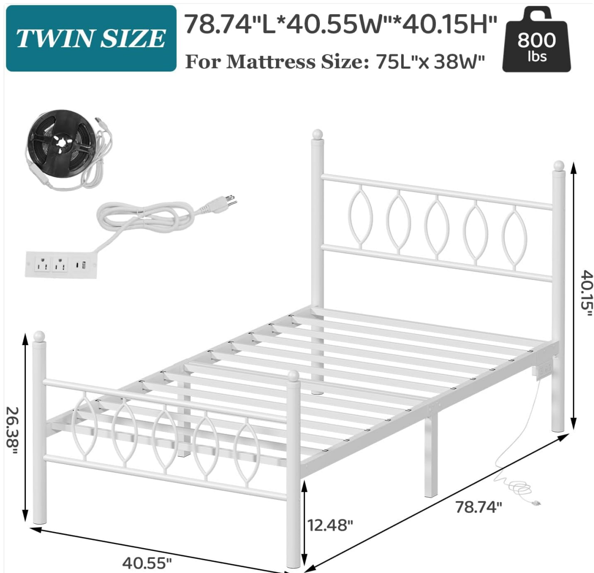
Image: Overview of bed frame components and dimensions.
