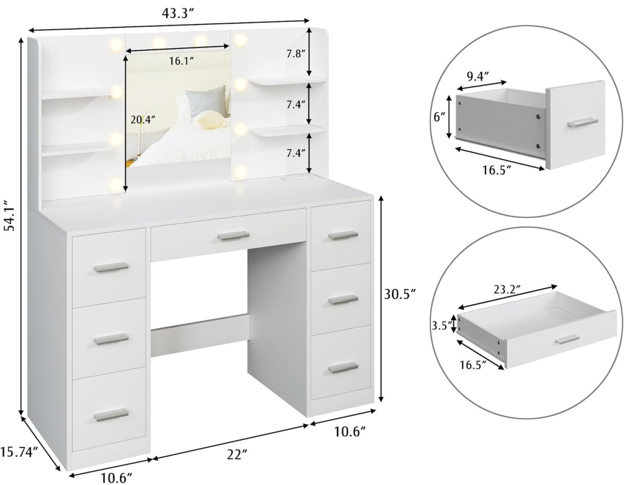
Figure 3.1: A detailed diagram illustrating the dimensions of the vanity desk, including the mirror, desktop, and drawers.
