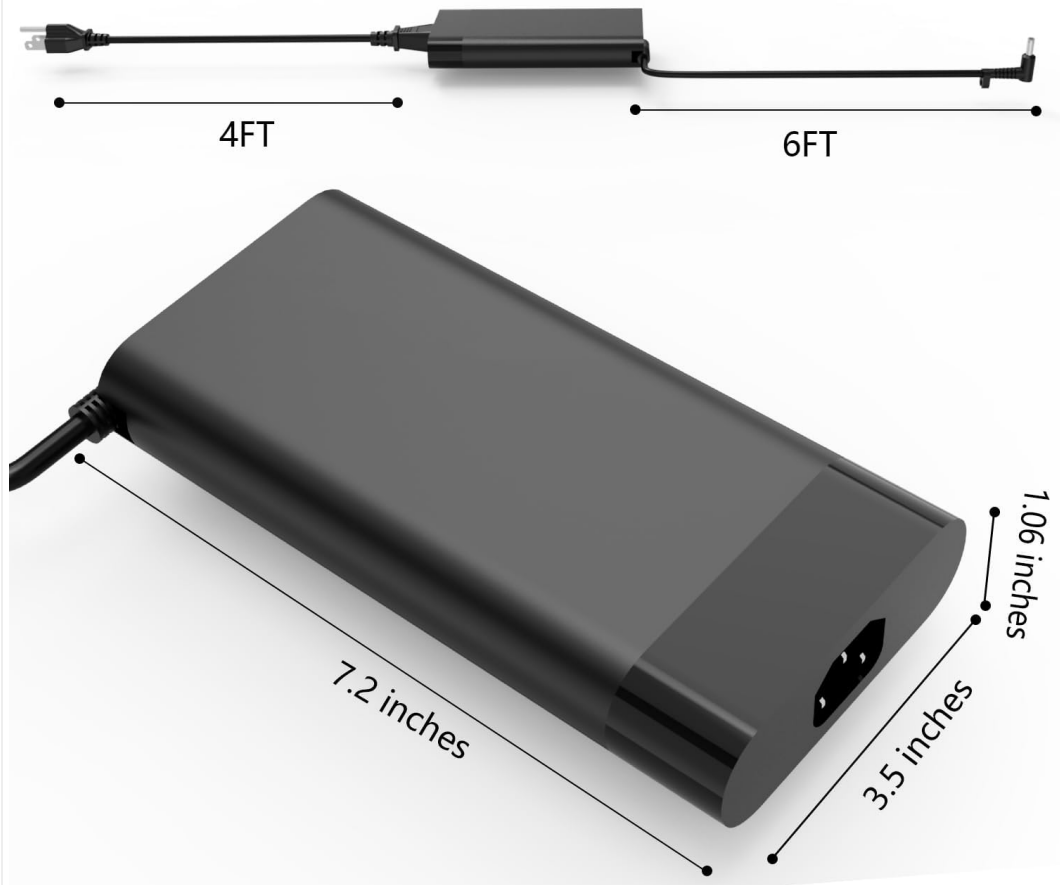
Image 8.1: Physical dimensions of the charger unit and cable lengths.
