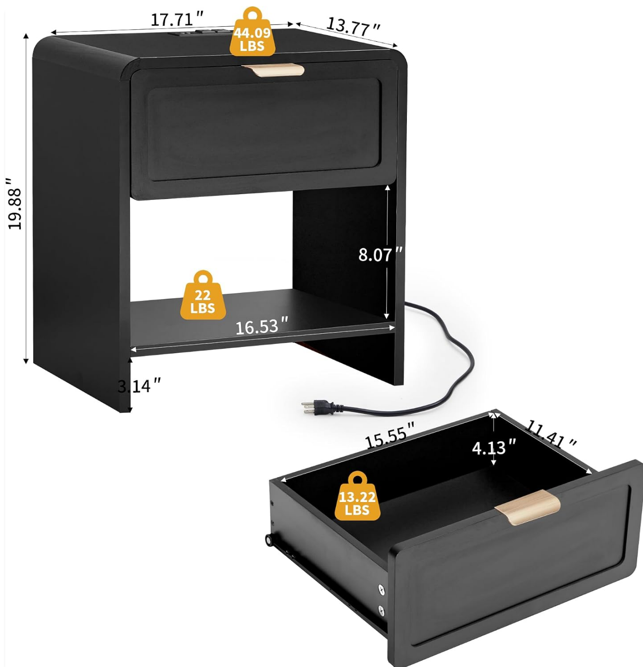
Image 9.1: Dimensional diagram of the nightstand, including overall size and internal measurements for the drawer and open shelf, along with weight capacities.
