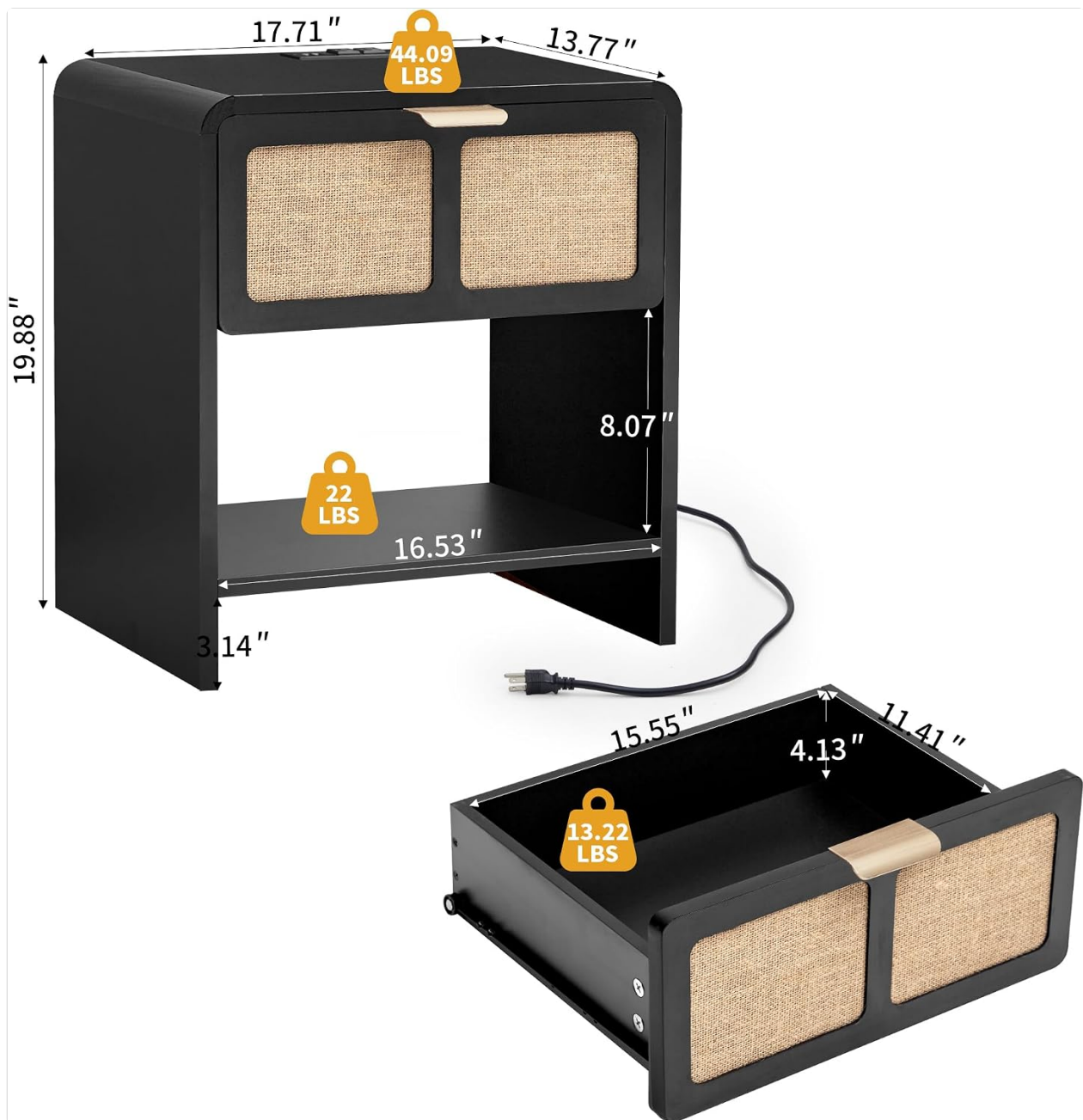
Image: Detailed view of the nightstand's dimensions and components, including the drawer and charging station.
