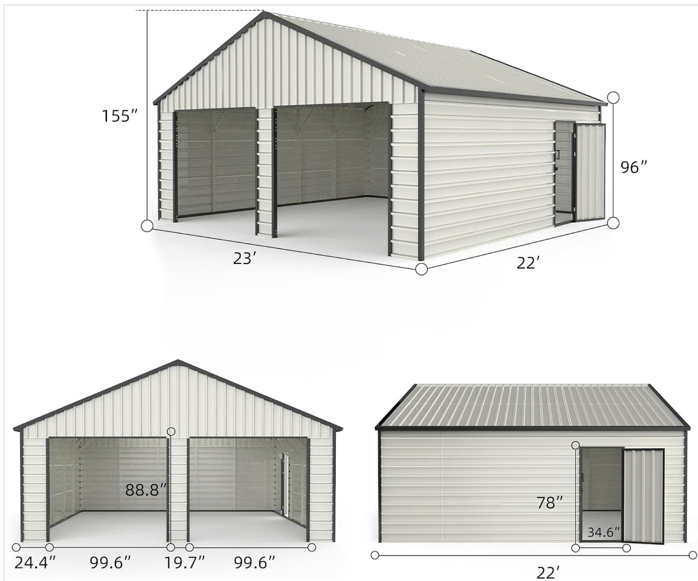
Image: Dimensional diagram of the ANTSKU Double Garage Metal Shed.
