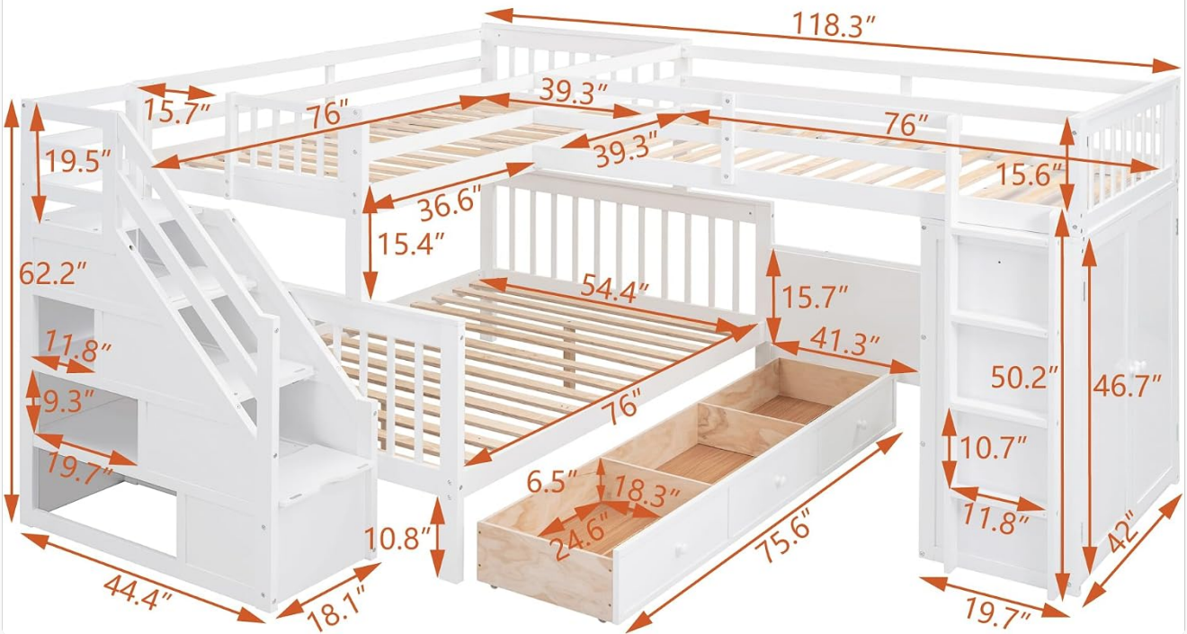
Image: Detailed dimensions of the Bellemave L-Shape Bunk Bed, showing measurements for each section including the twin beds, full bed, staircase, wardrobe, and drawers.
