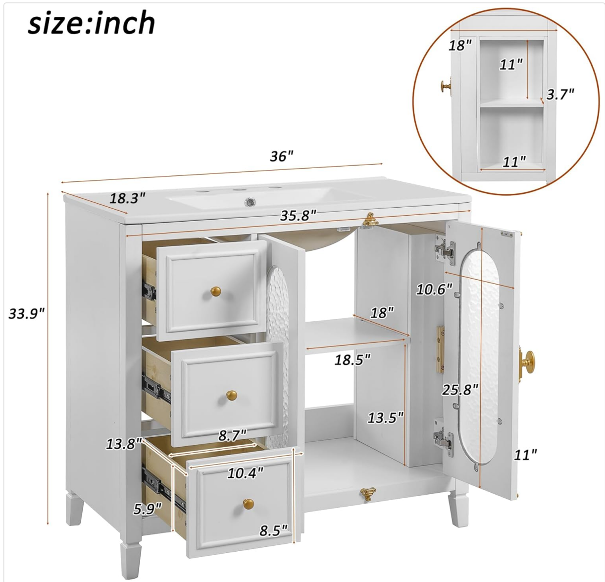
Image: Detailed dimensional drawing of the vanity, showing internal measurements for drawers, cabinet, and side storage.
