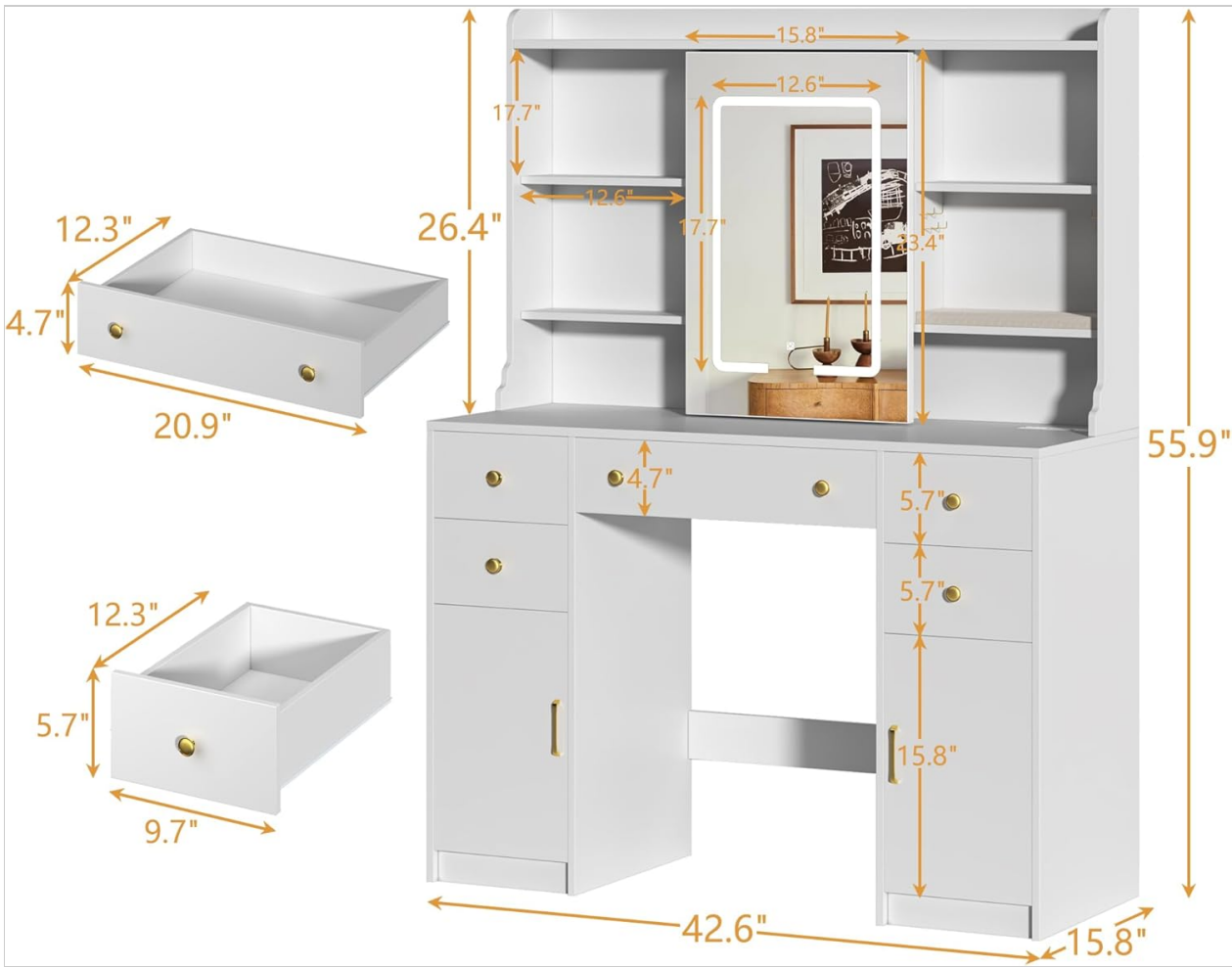
Image 8.1: Dimensional diagram of the HUAHUU Vanity Desk.
