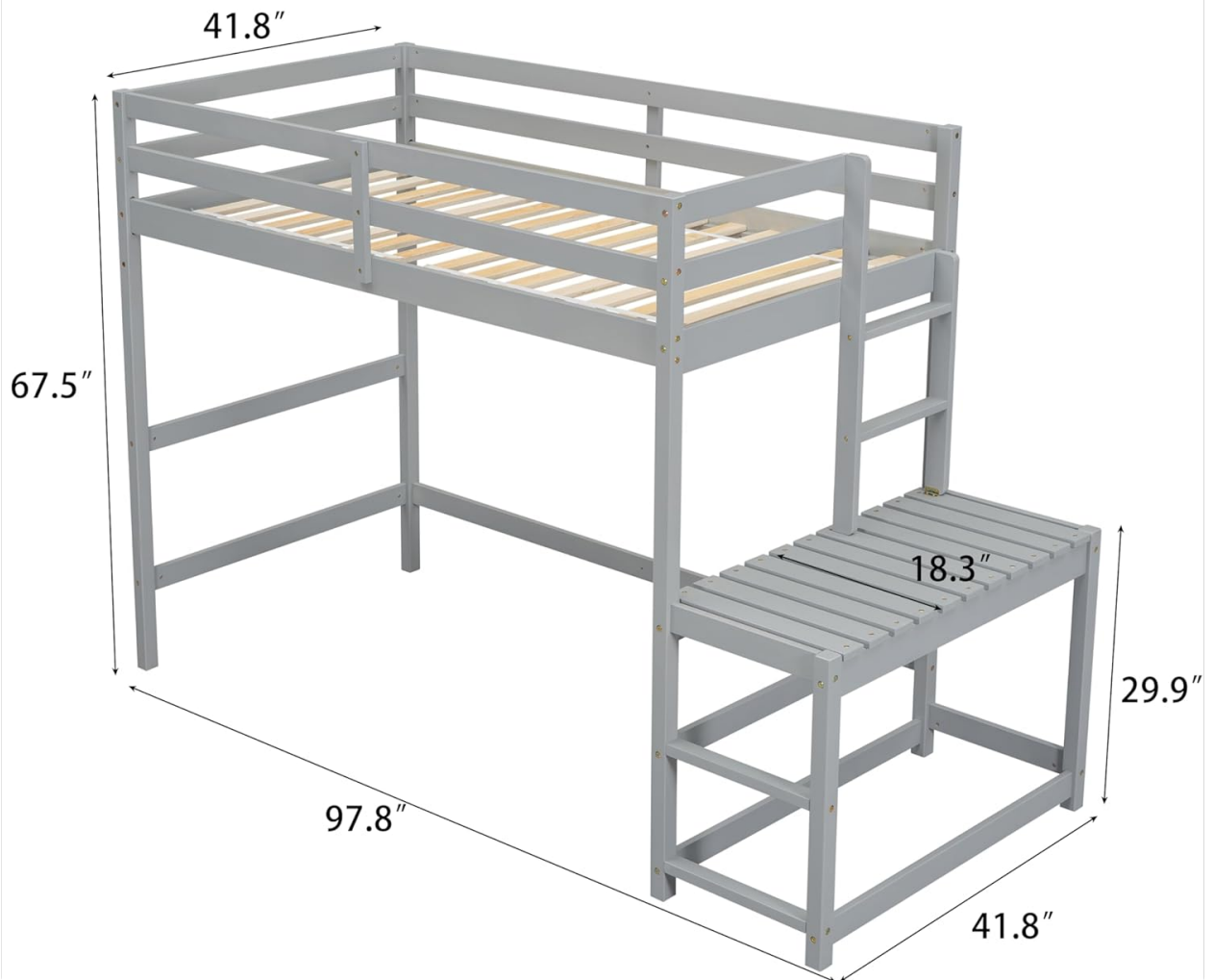
Image: A detailed diagram illustrating the key dimensions of the LINKHOO Twin High Loft Bed, including its overall length, width, and height, as well as the height of the landing platform.
