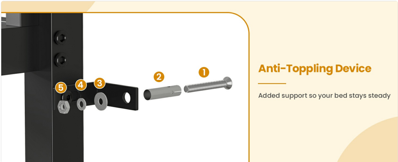
Figure 2.1: Illustration of the anti-topping device components and their installation to ensure bed stability.
