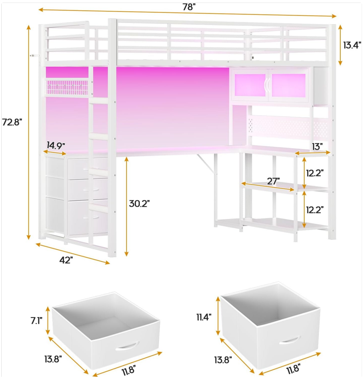
Figure 4.2: Product dimensions for planning and assembly.
