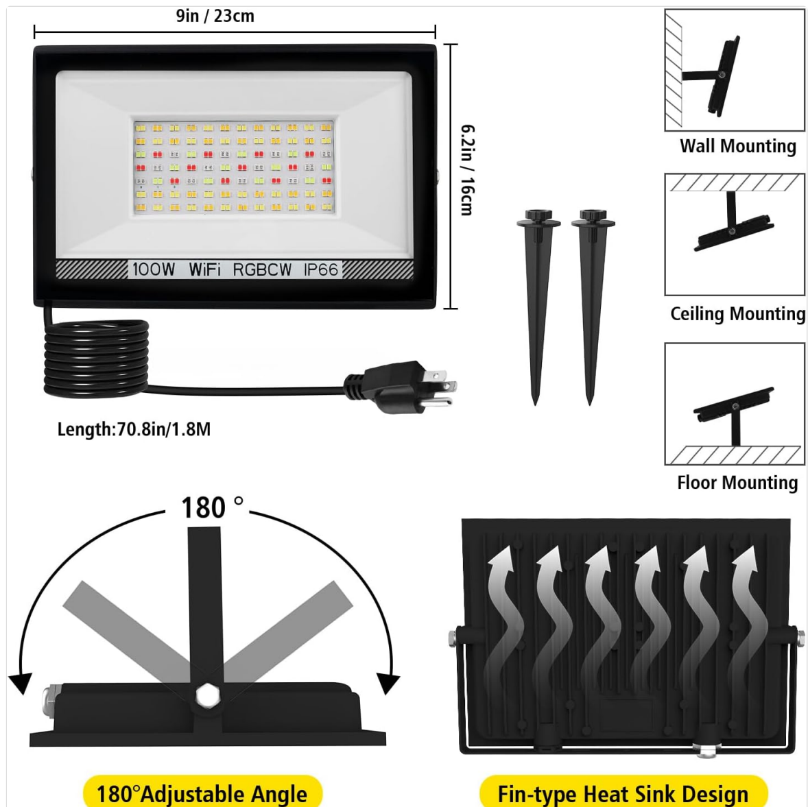
Image 5.1: Product dimensions and mounting options.
