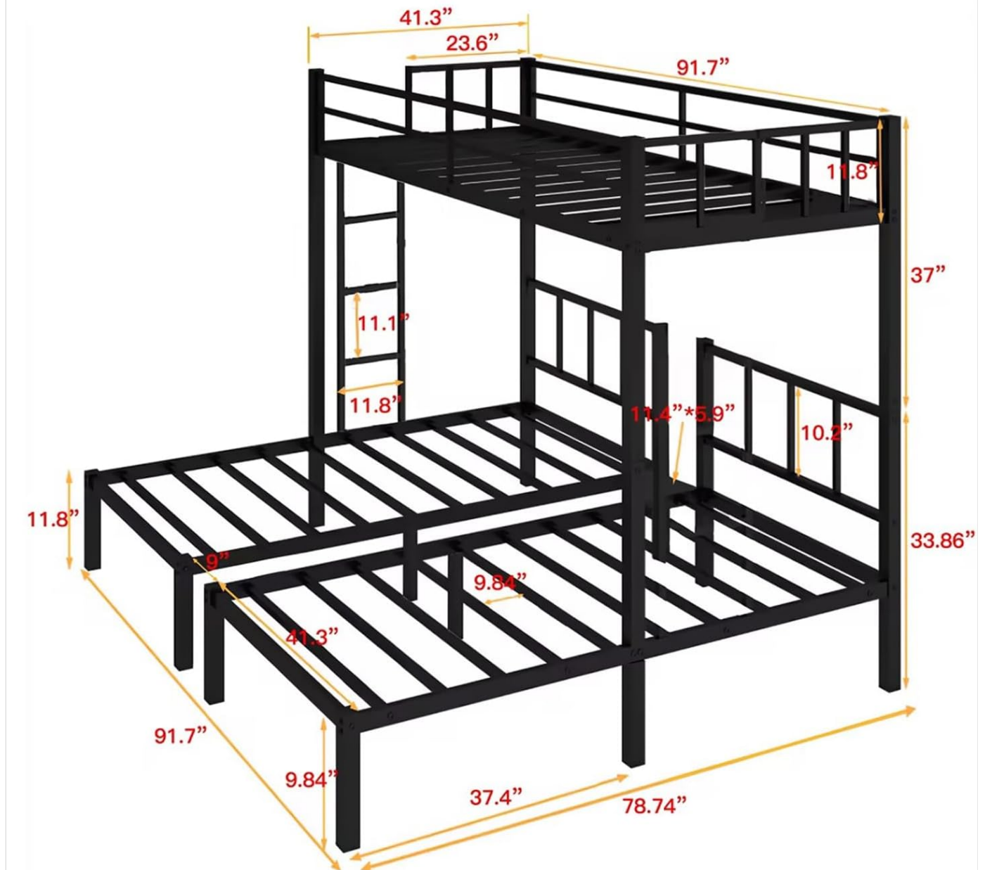
Image: A comprehensive diagram illustrating the dimensions of the Zevemomo Triple Bunk Bed, including the length, width, and height of the upper and lower beds, and overall structure.
