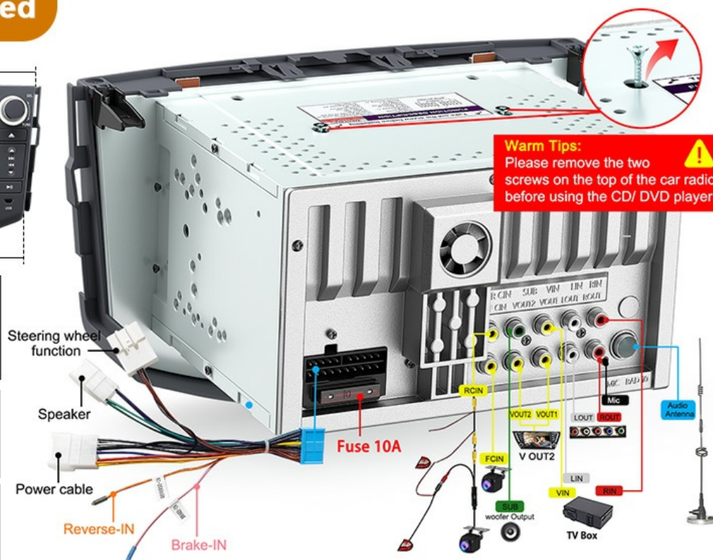
Image: Wiring diagram and physical dimensions of the car radio unit.
