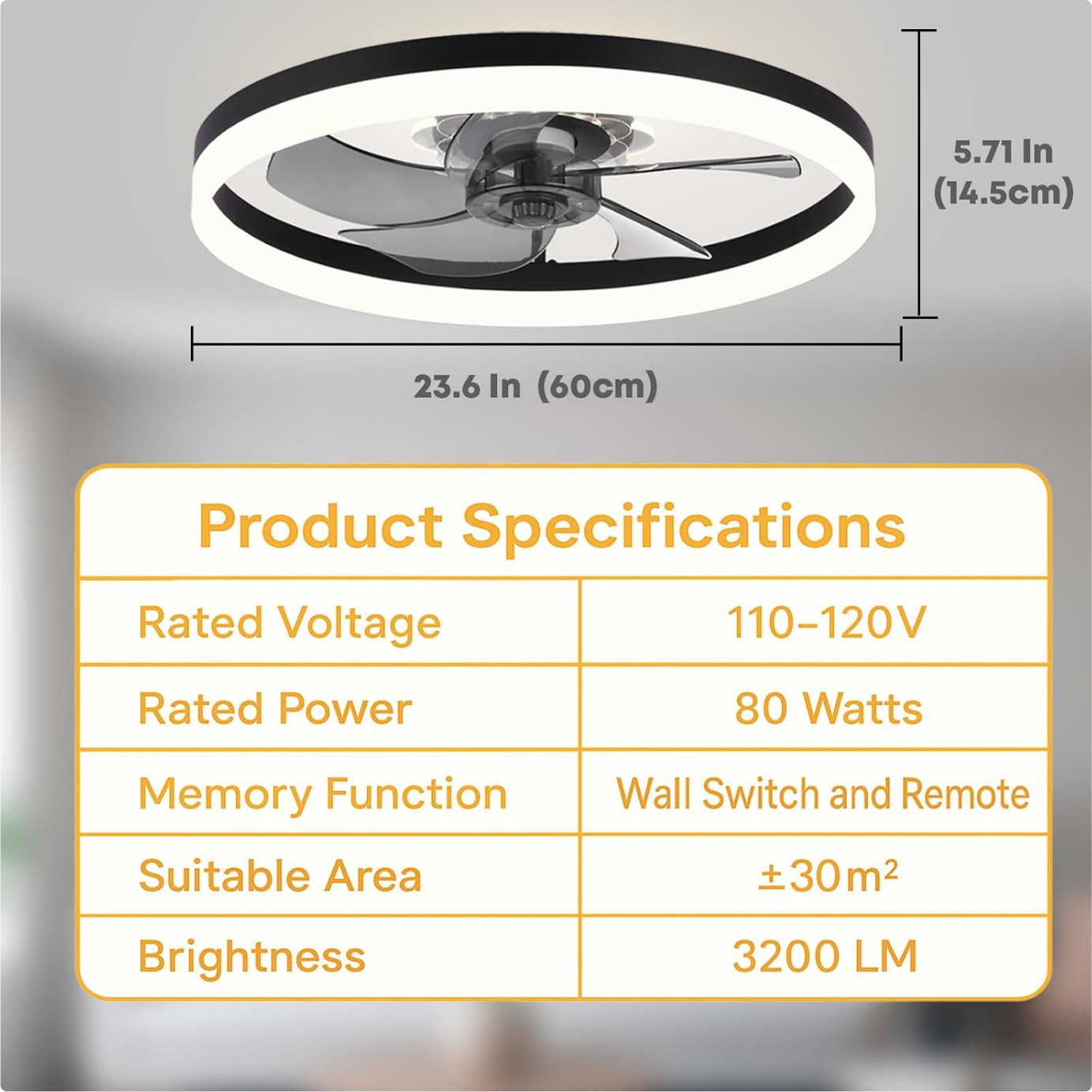
Image 4.1: Overview of product dimensions and key electrical specifications.
