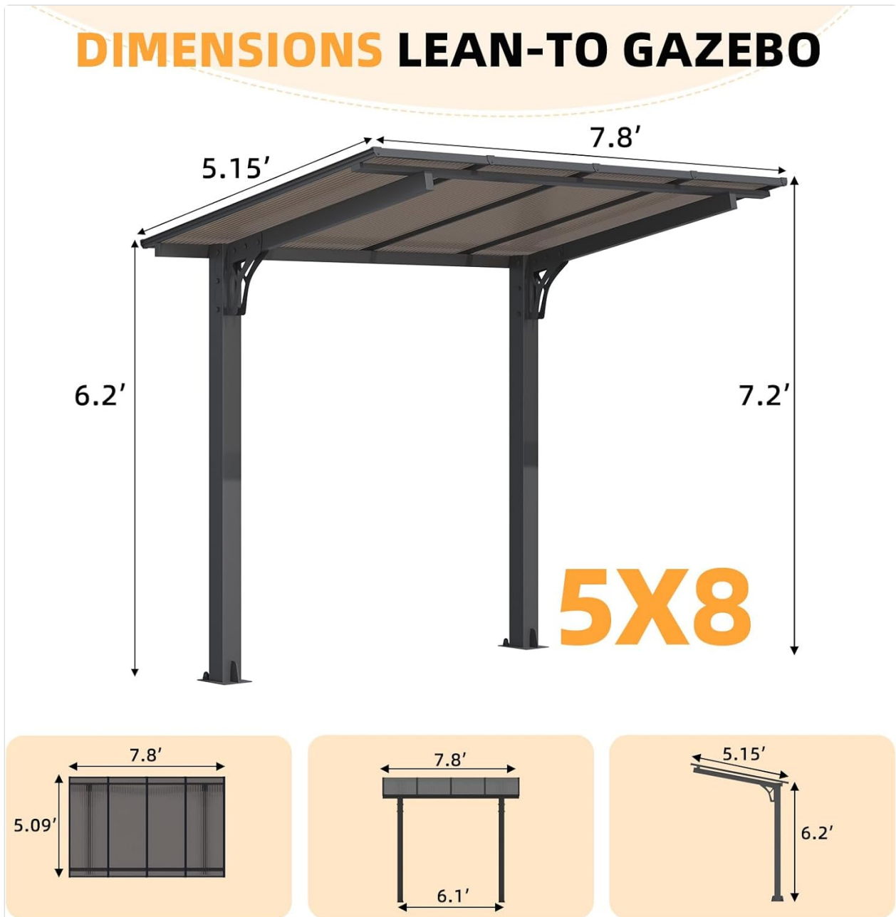
Figure 2.2.1: AECOJOY 5x8 Grill Gazebo Dimensions. The diagram illustrates the overall length of 7.8 feet, width of 5.15 feet, and heights of 6.2 feet and 7.2 feet at different points.
