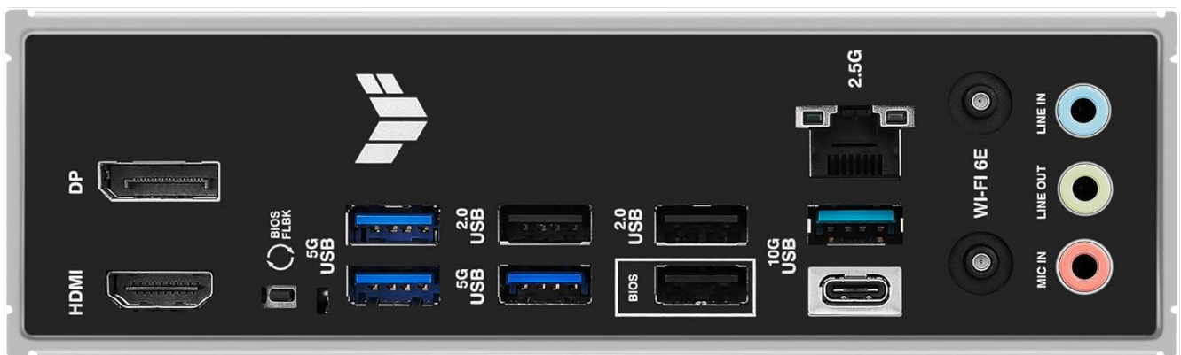
Figure 4.2: Rear I/O panel with various ports including USB, DisplayPort, HDMI, 2.5G LAN, and Wi-Fi 6E antenna connectors.
