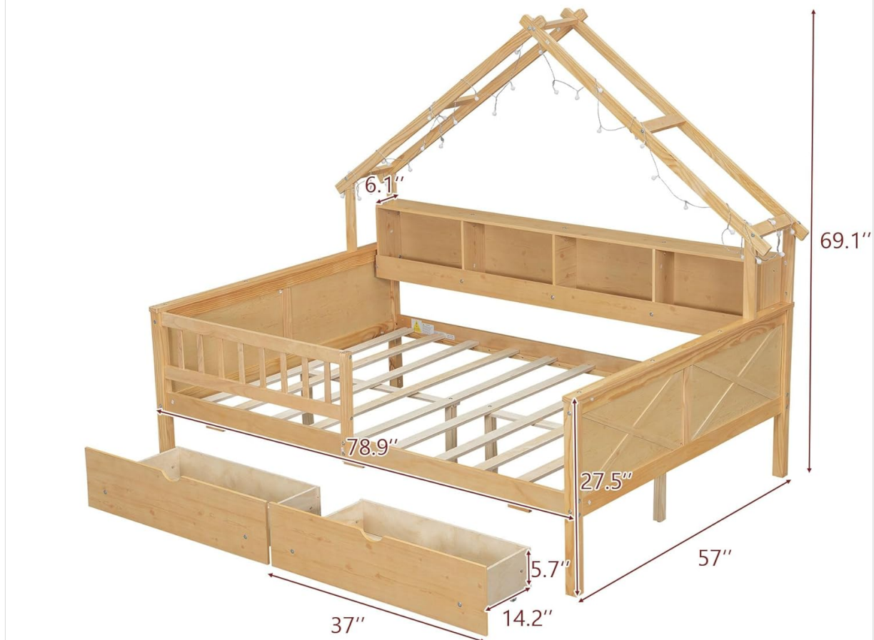
Figure 4: Product Dimensions
