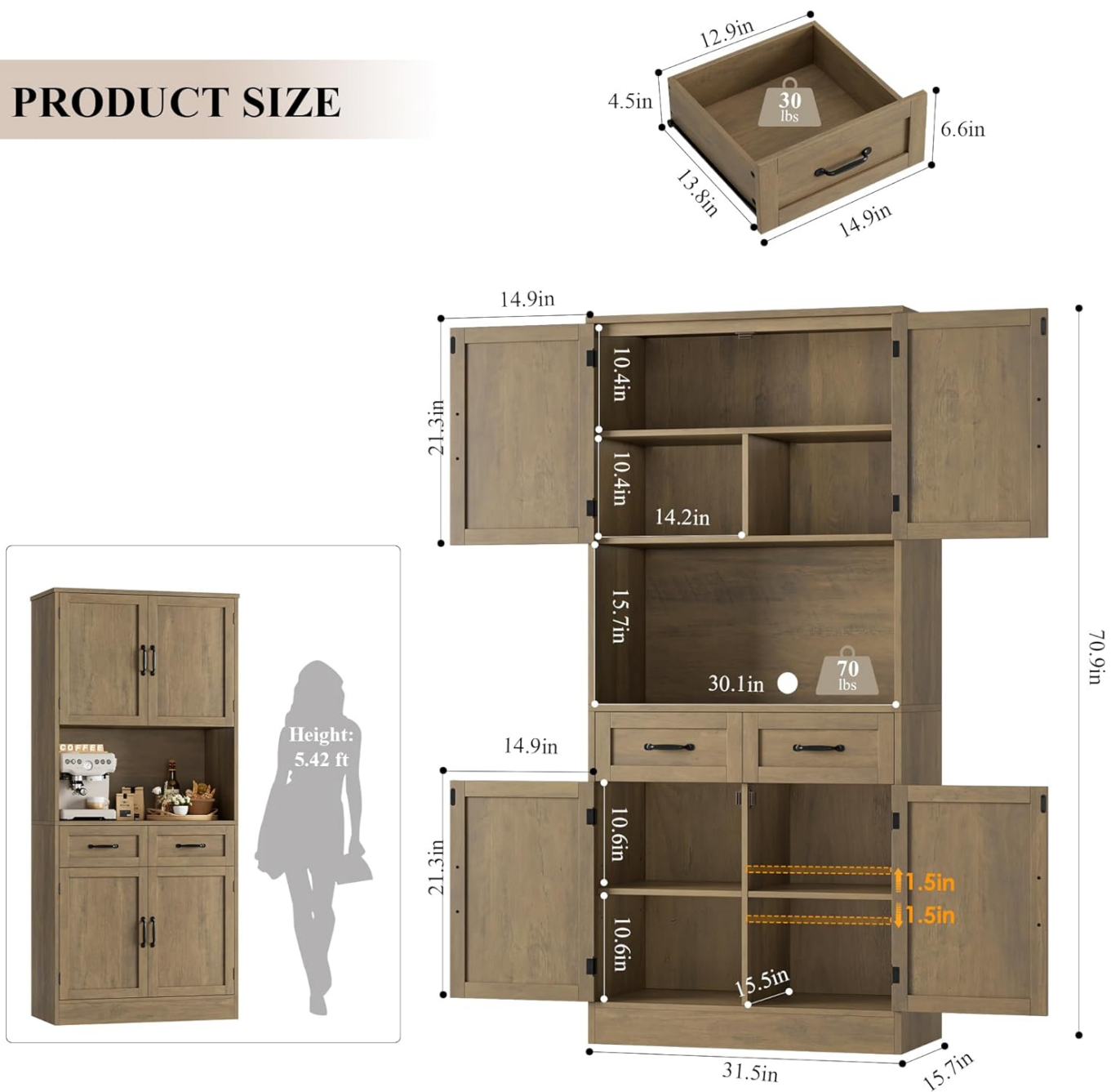
Figure 2: Product dimensions and internal structure for assembly reference.
