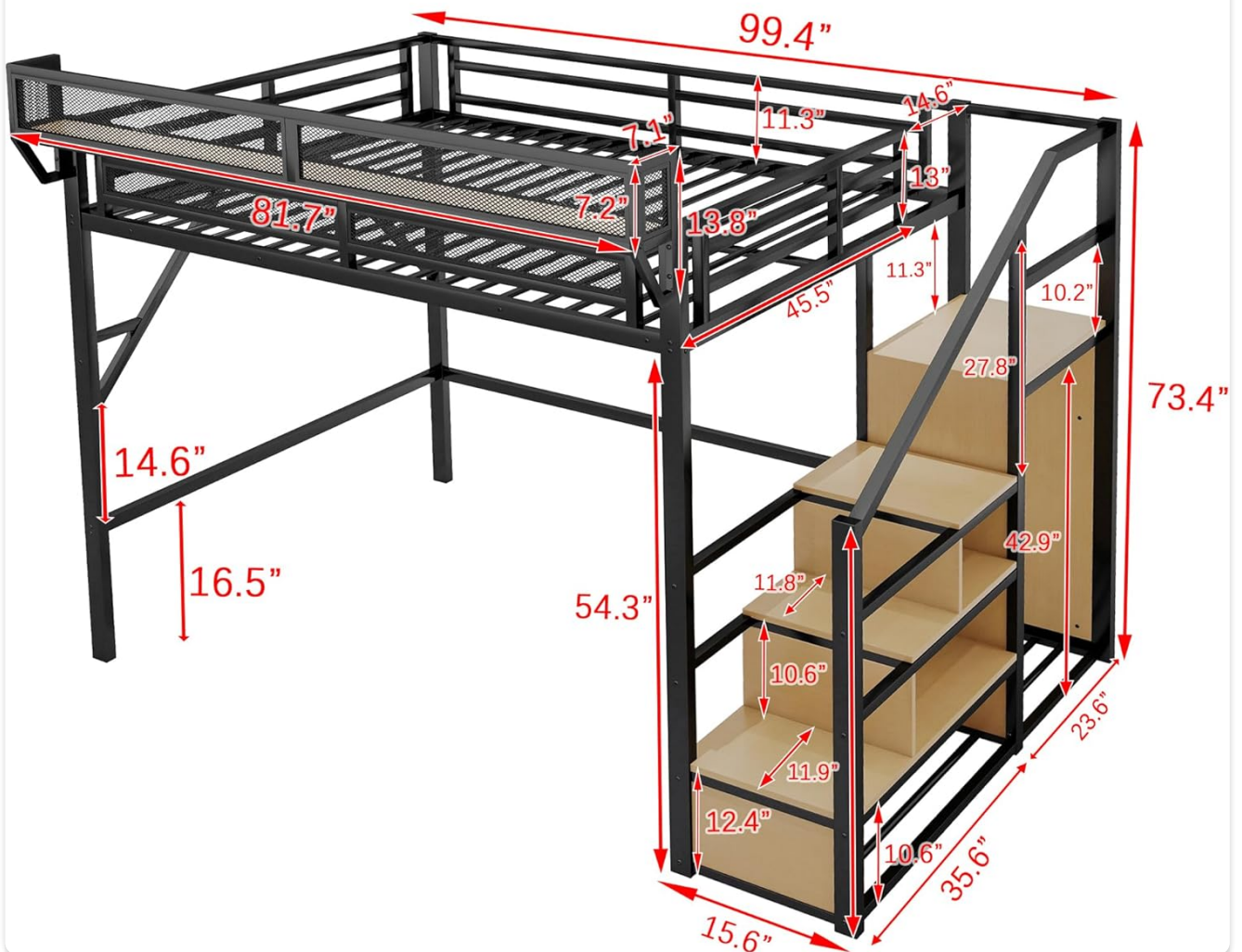
Image: A detailed diagram illustrating the key dimensions of the KEIKI Queen Size Metal Loft Bed Frame, including length, width, height, and under-bed clearance.
