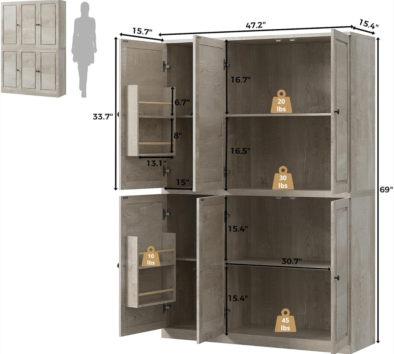
Figure 2: Product Dimensions and Internal Layout. This diagram provides a detailed view of the cabinet's dimensions (15.4"D x 47.2"W x 69"H) and internal shelf configurations, including weight capacities for different sections.
