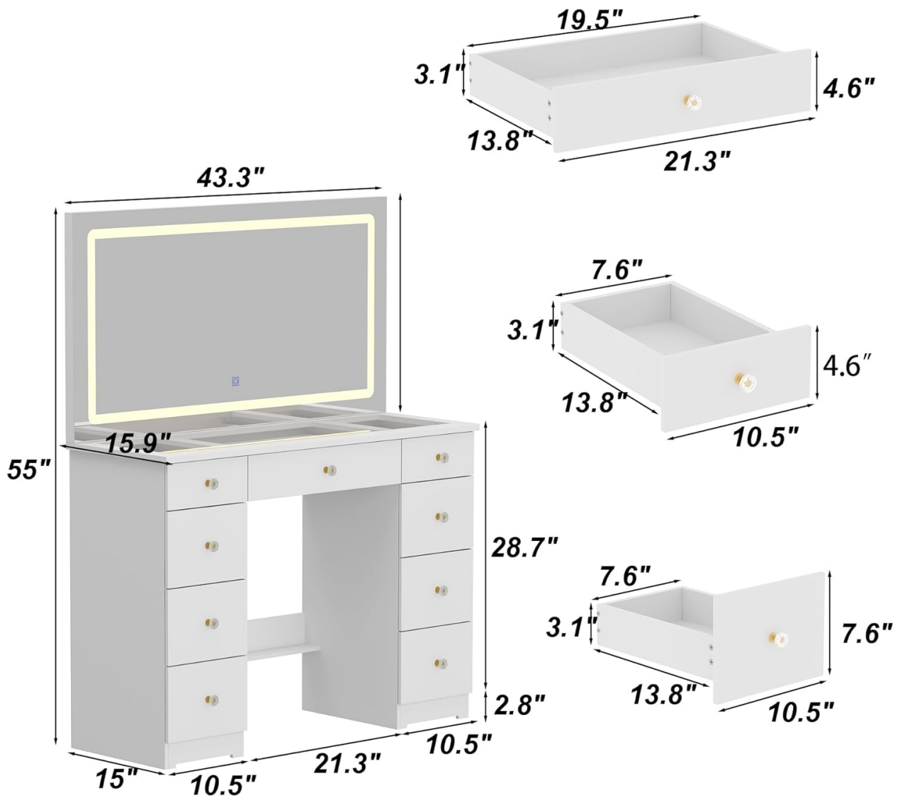
Figure 7.1: Detailed dimensions of the vanity desk and its individual drawers.
