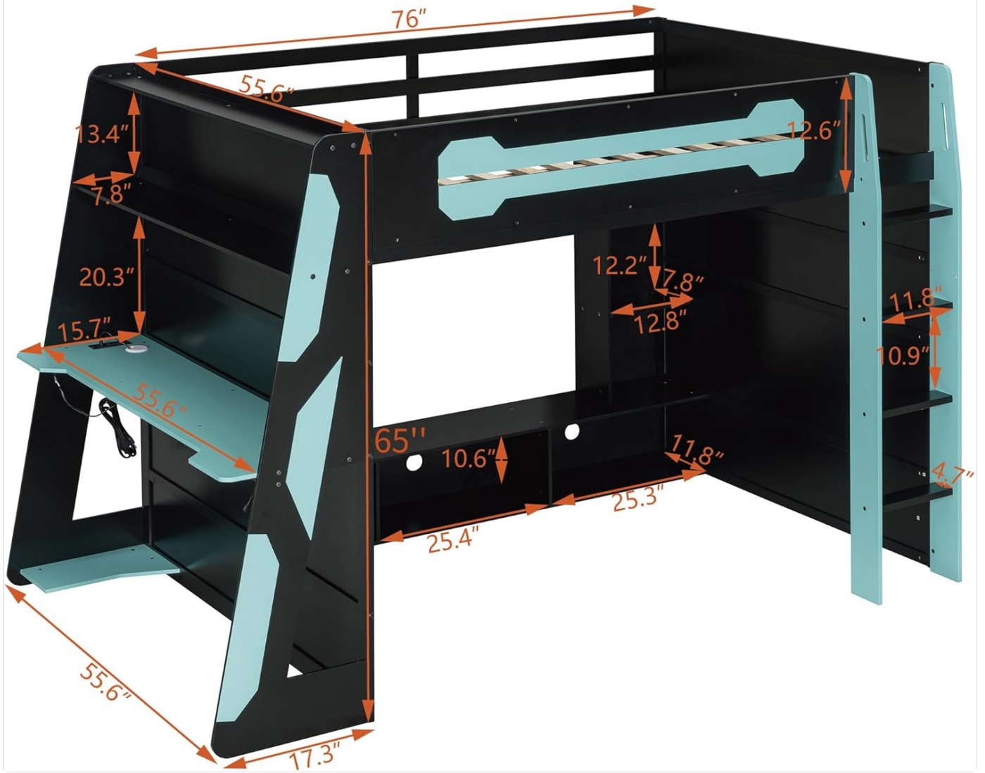
Image: Overall dimensions of the Bellemave Full Size Wood Gaming Loft Bed with Desk.
