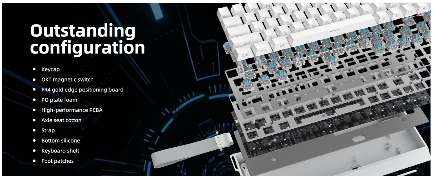
Image: An exploded diagram illustrating the internal components of the IROK Mer68 SE keyboard, including keycaps, magnetic switches, and PCB.
