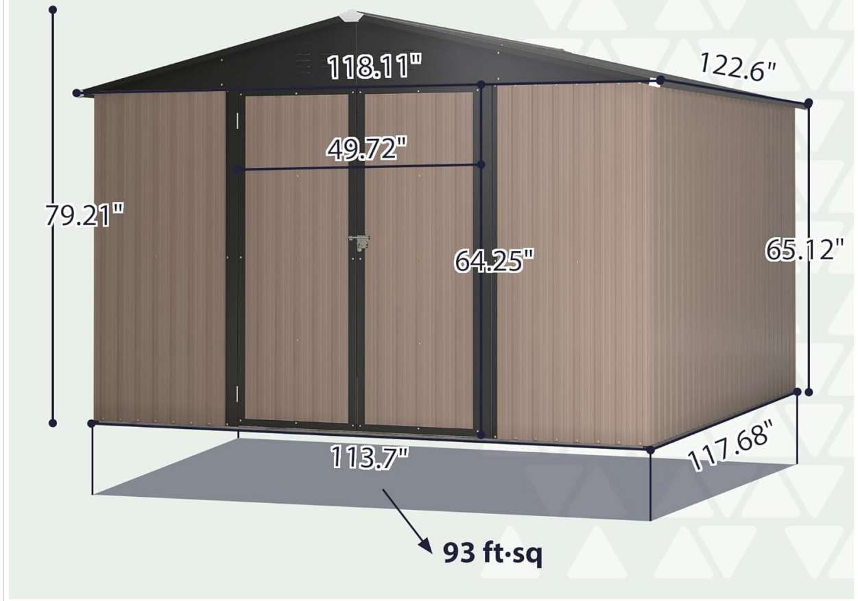
Image 4.2: A diagram illustrating the key dimensions of the cattino 10x10 FT Outdoor Storage Shed, including length (113.70 in), width (117.68 in), and height (79.21 in). This is crucial for planning the installation site.
