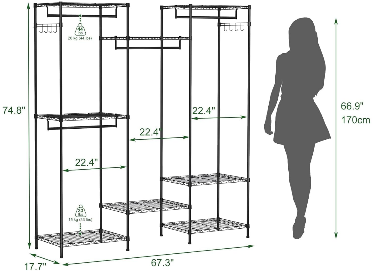
Figure 8.1: Detailed product dimensions and weight capacities.
