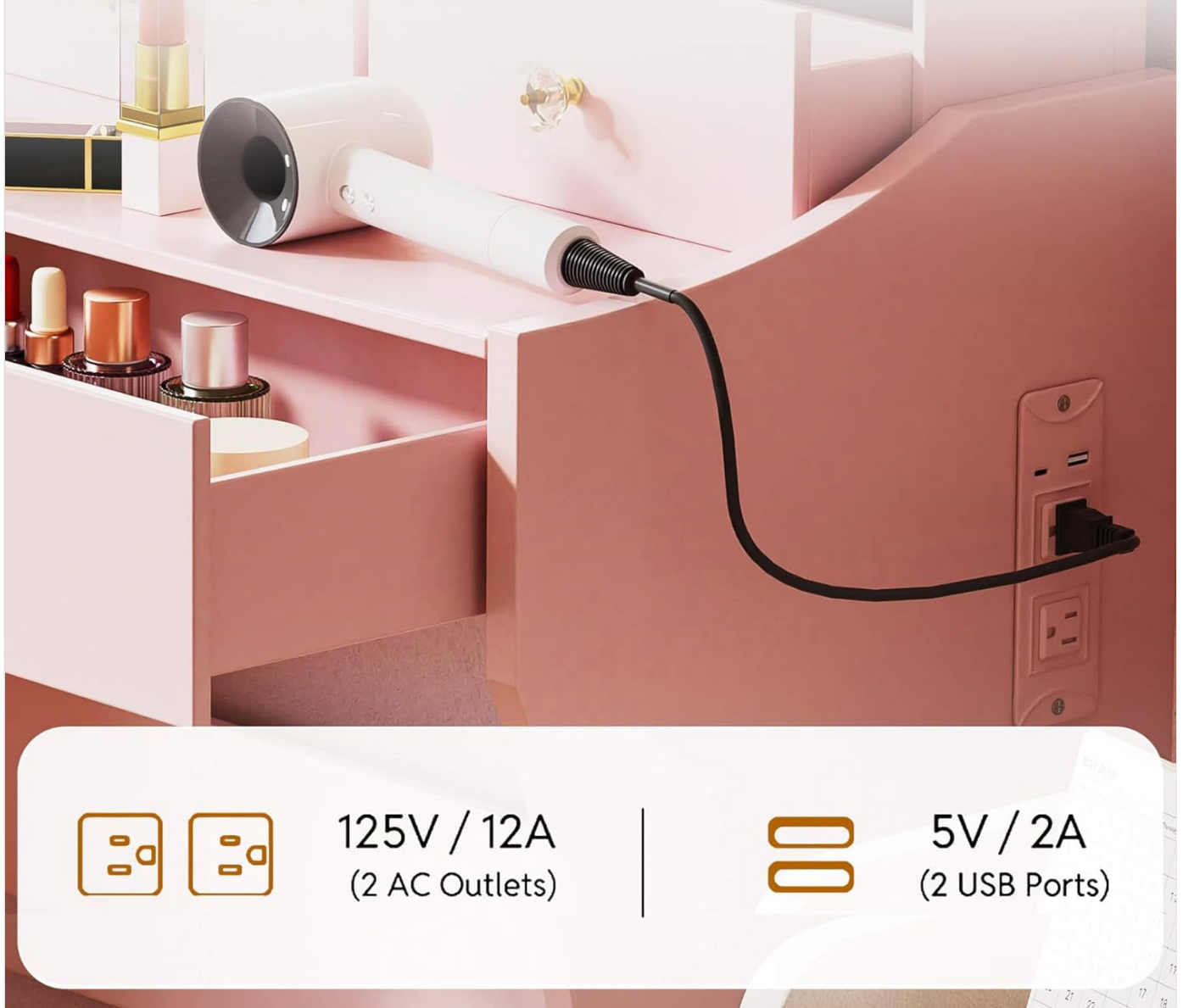
Image 5.2: Close-up of the integrated charging station.
