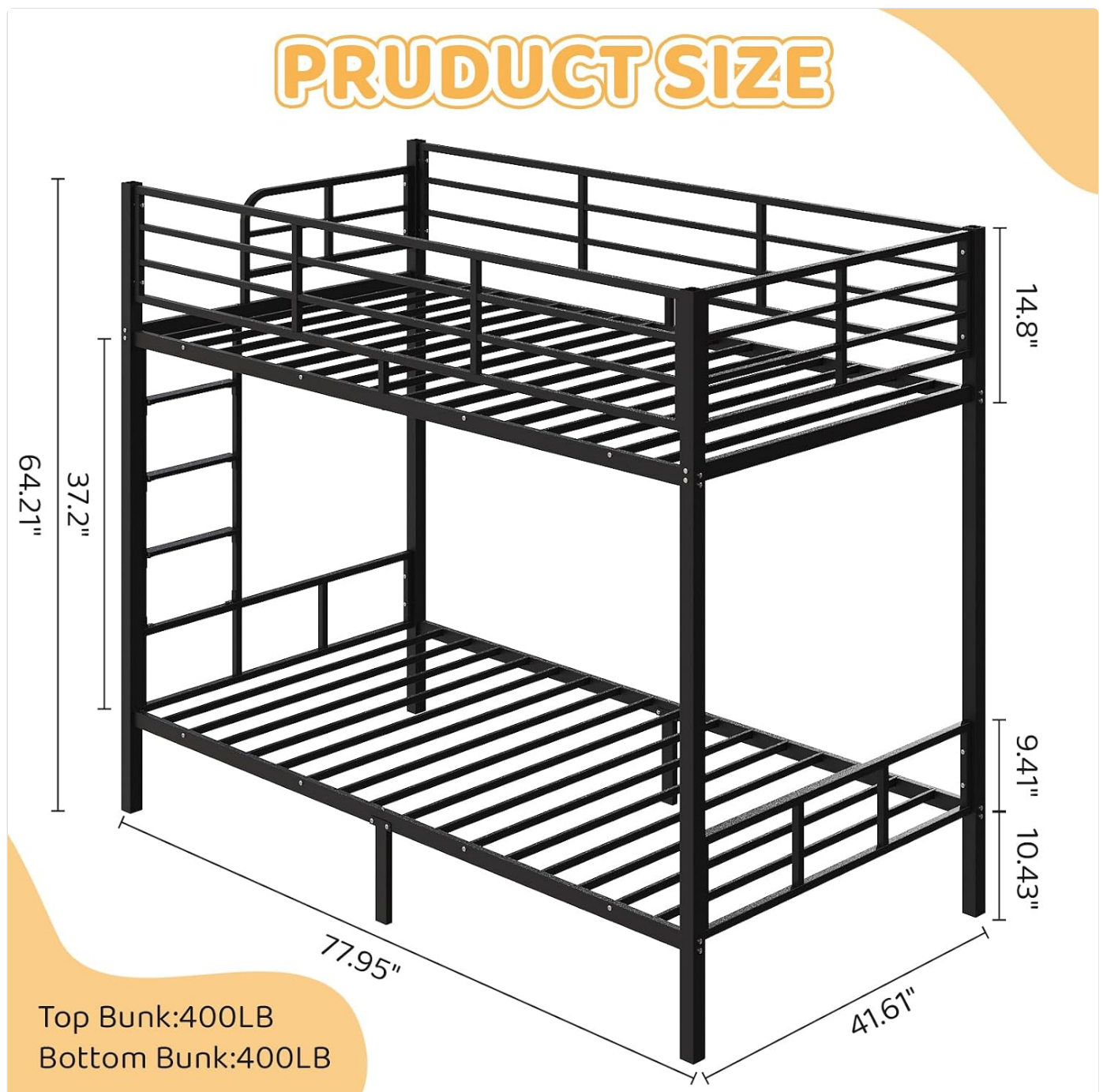
Figure 6: Detailed product dimensions and weight capacity.
