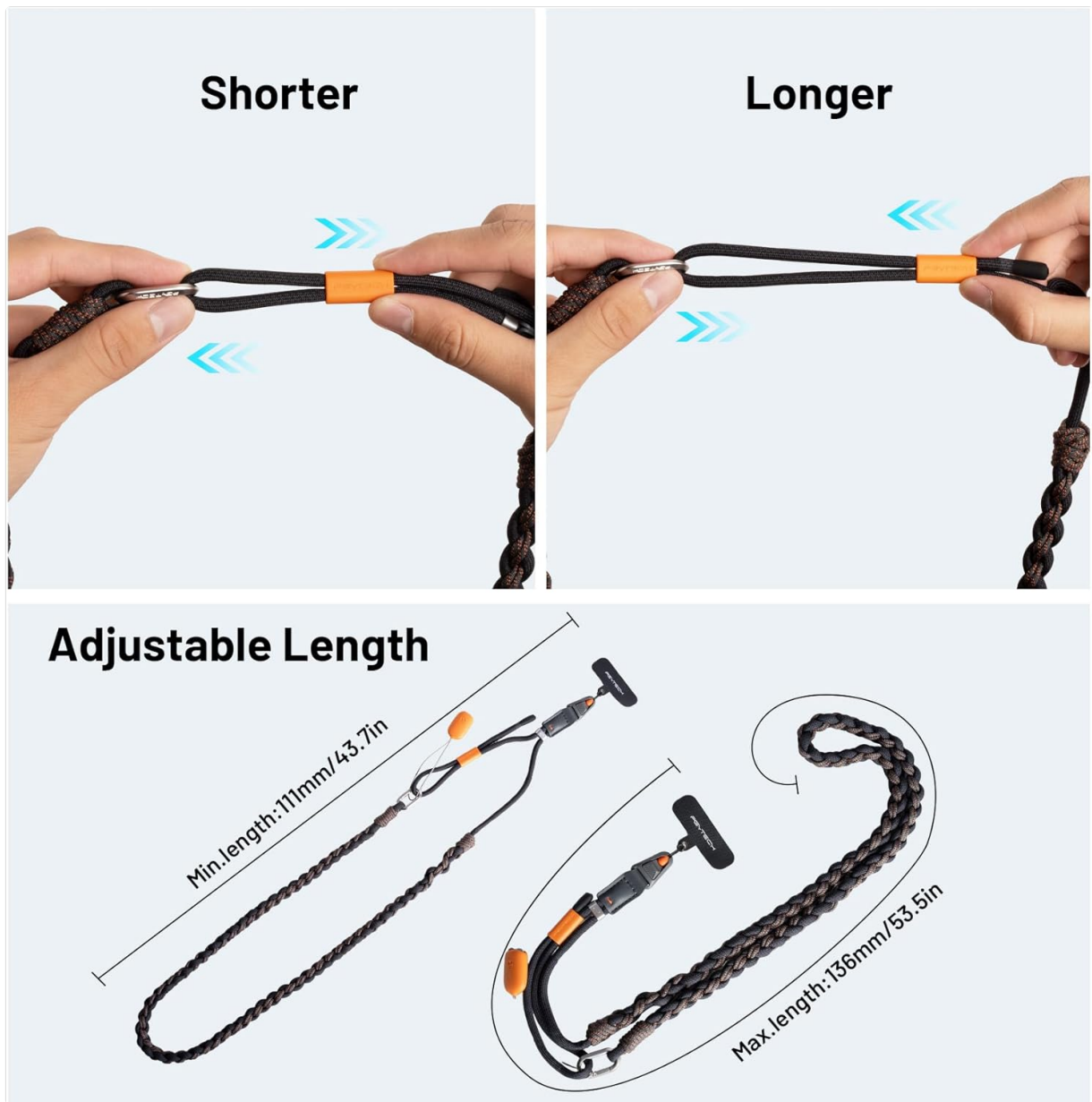
Figure 5: Strap Length Adjustment. This image shows how to shorten or lengthen the strap and its adjustable range.
