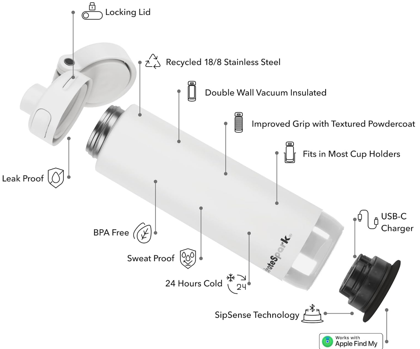
Figure 6: Exploded view highlighting key components and features for maintenance.
