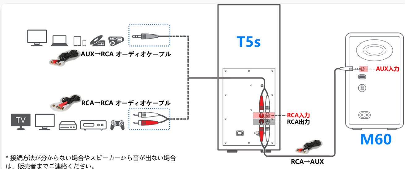
Figure 5: Connection diagram illustrating the setup of the Edifier T5s Subwoofer with Edifier M60 speakers, utilizing RCA connections.
