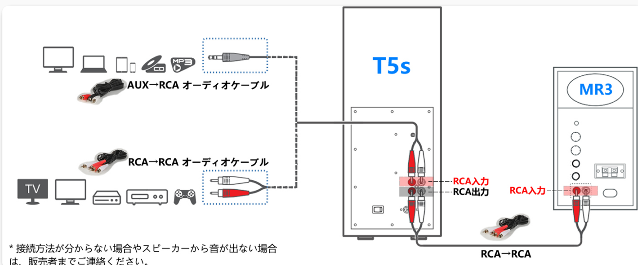
Figure 6: Connection diagram demonstrating how to connect the Edifier T5s Subwoofer to Edifier MR3 speakers using RCA cables.
