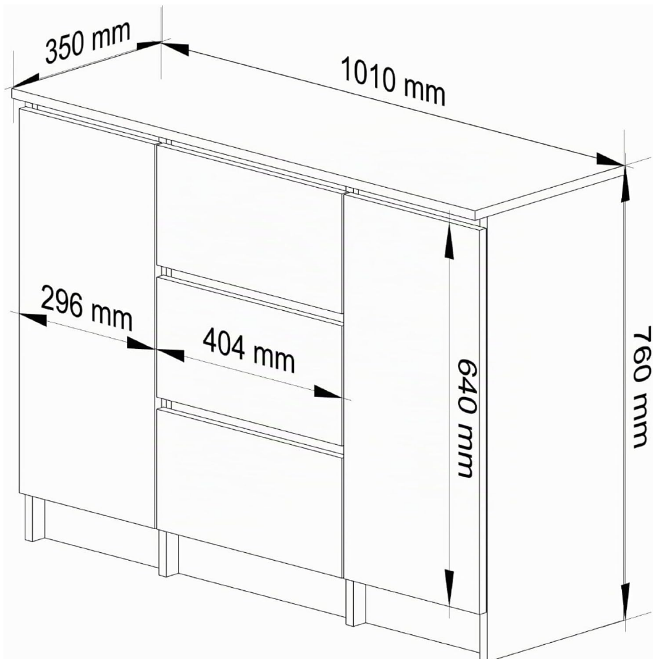
Image: Technical drawing illustrating the dimensions of the AKORD K-100 Chest of Drawers.
