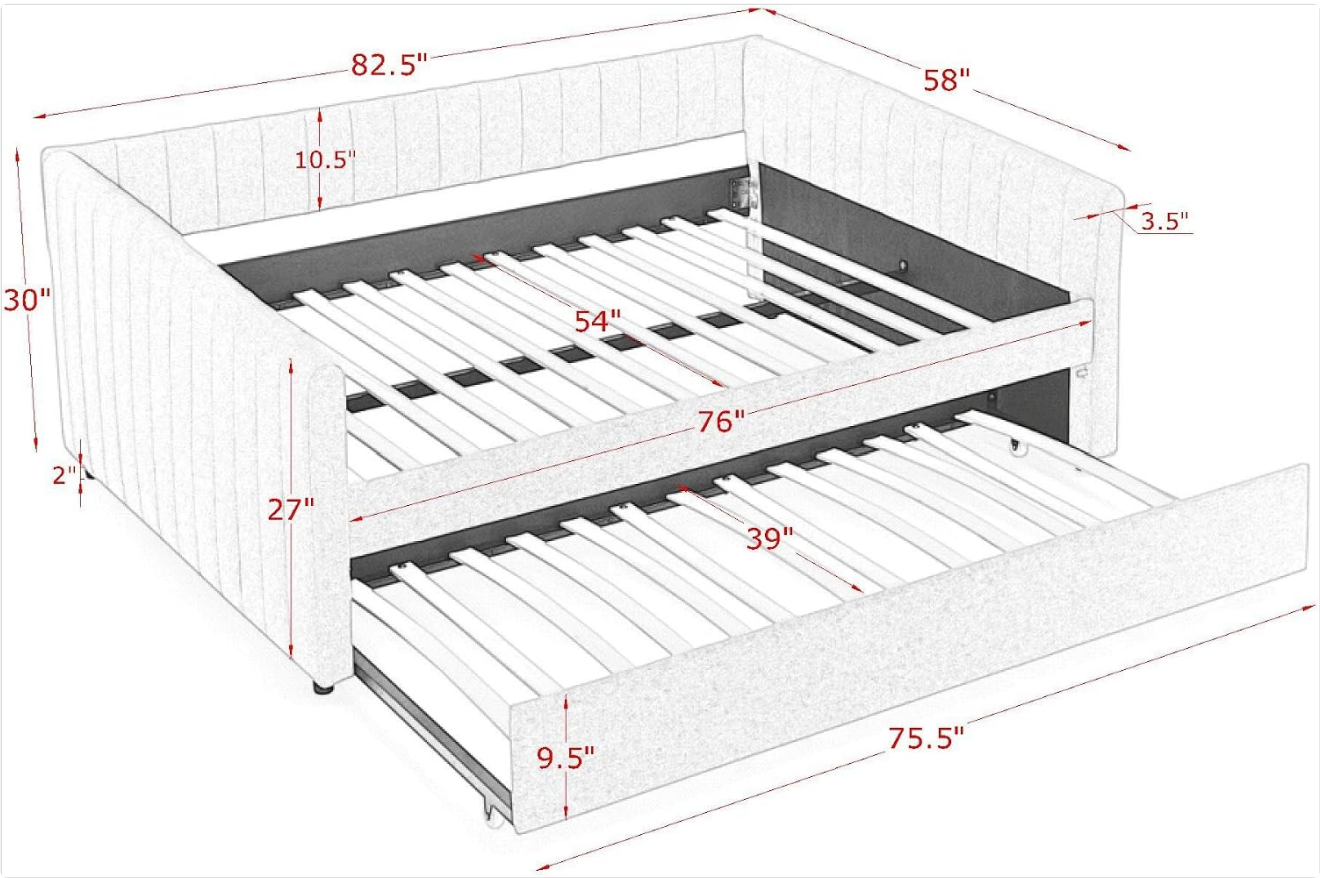
Image: Dimensional diagram of the daybed and trundle.
