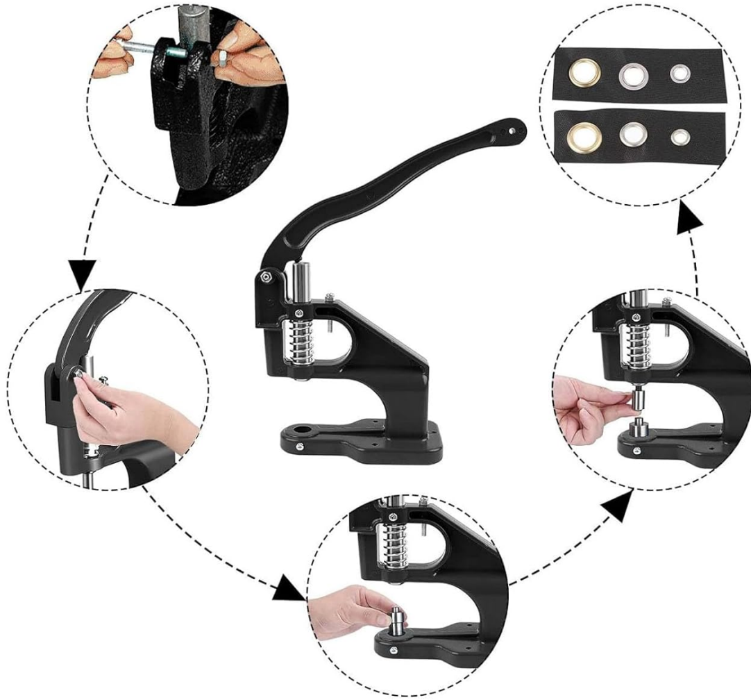
Figure 5.1: Visual guide on the operational steps, from preparing the material to pressing the grommet.
