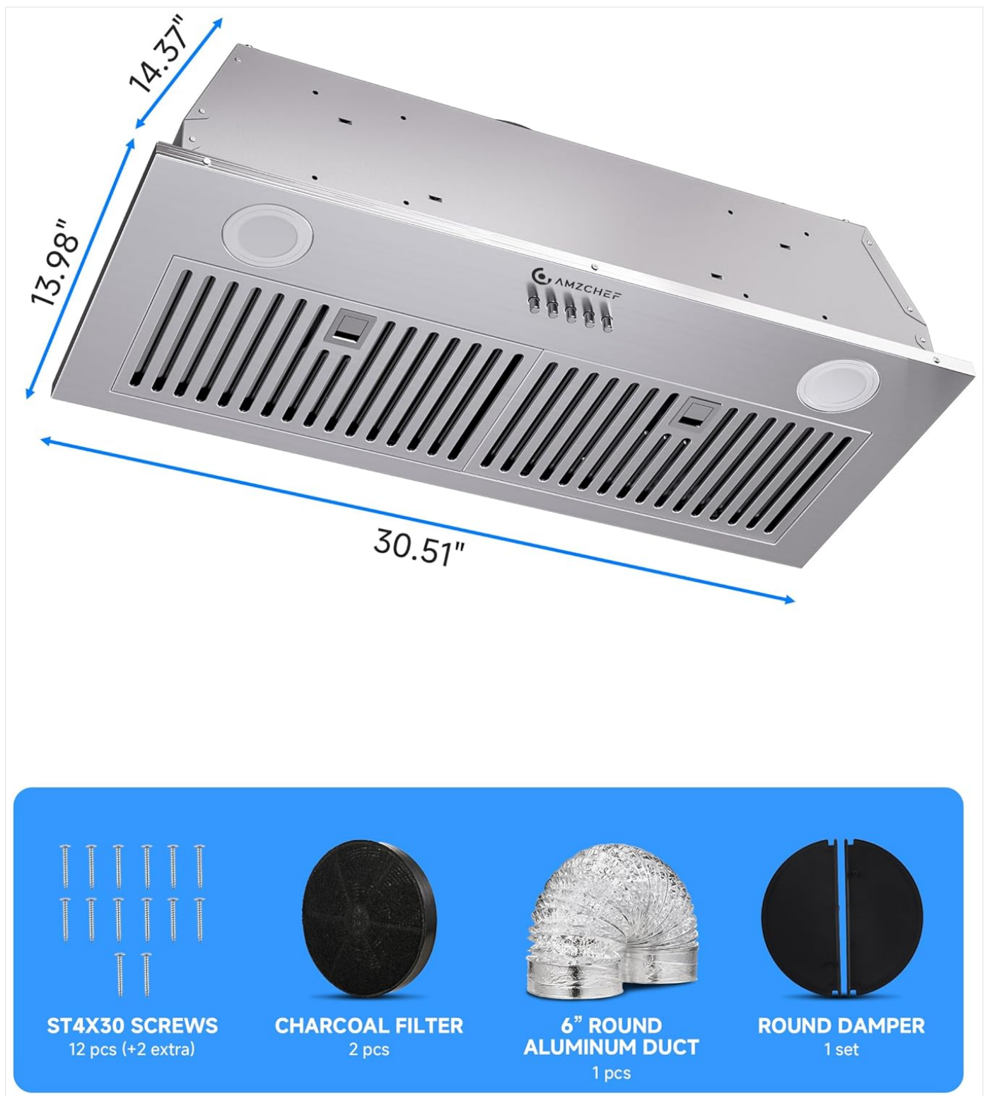
Figure 3.1: Included components for the AMZCHEF Range Hood Insert, showing the main unit, baffle filters, charcoal filters, 6-inch aluminum duct, round damper, and mounting screws.
