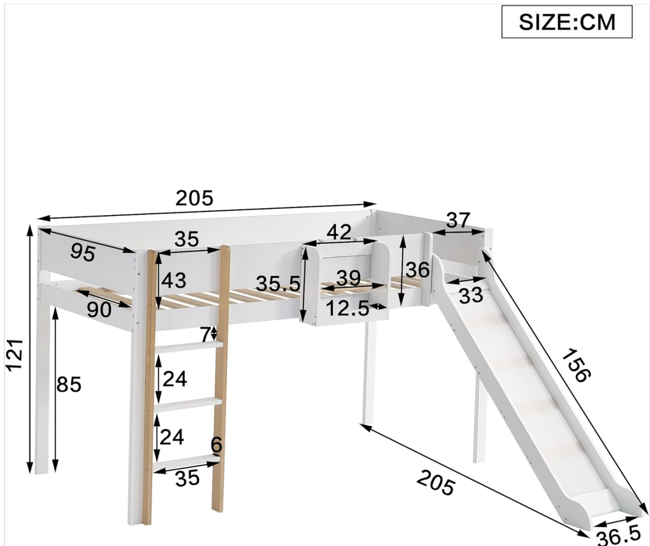
Figure 1: Dimensions diagram of the Merax Loft Bed. This image shows the overall length (205cm), width (95cm), and height (121cm) of the bed frame, along with detailed measurements for the ladder, slide, and integrated shelf. All measurements are in centimeters.
