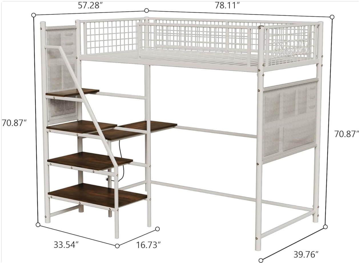
Figure 4: Product dimensions overview.
