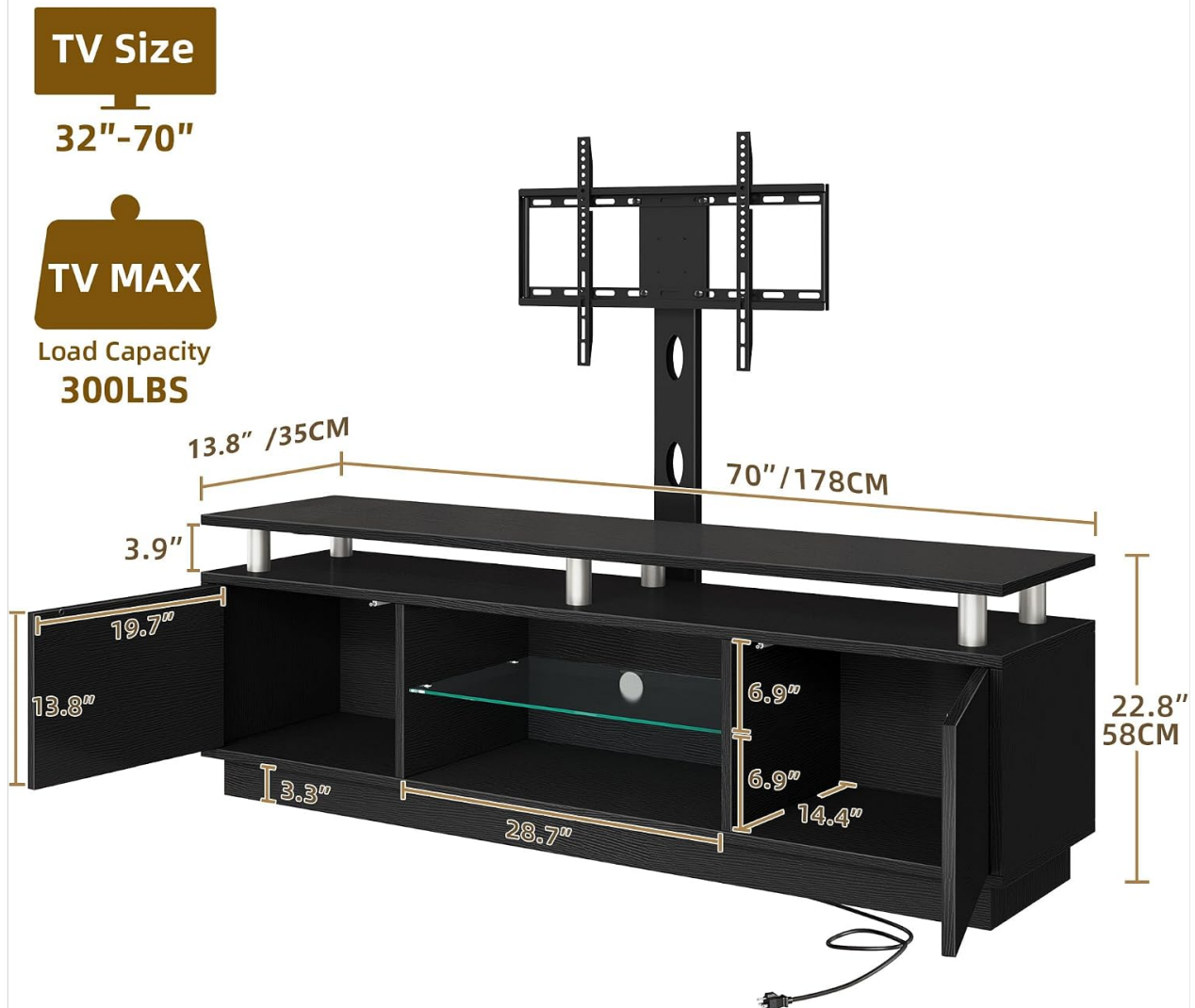
Figure 1: Product Dimensions. This diagram illustrates the overall dimensions of the TV stand and its various compartments, including the TV size compatibility (32"-70") and maximum load capacity (300 lbs).
