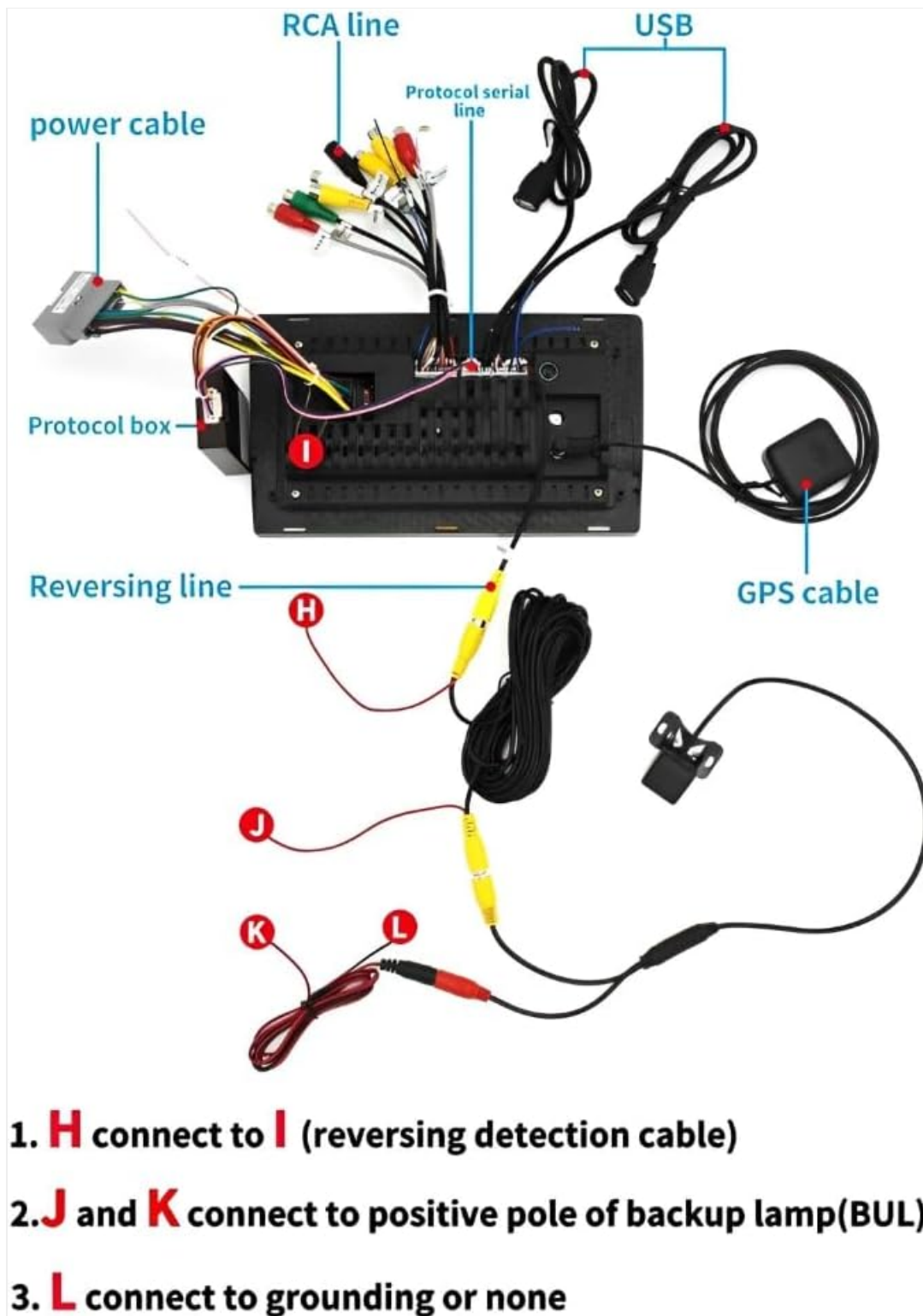
Image: Detailed wiring connections for the car radio.
