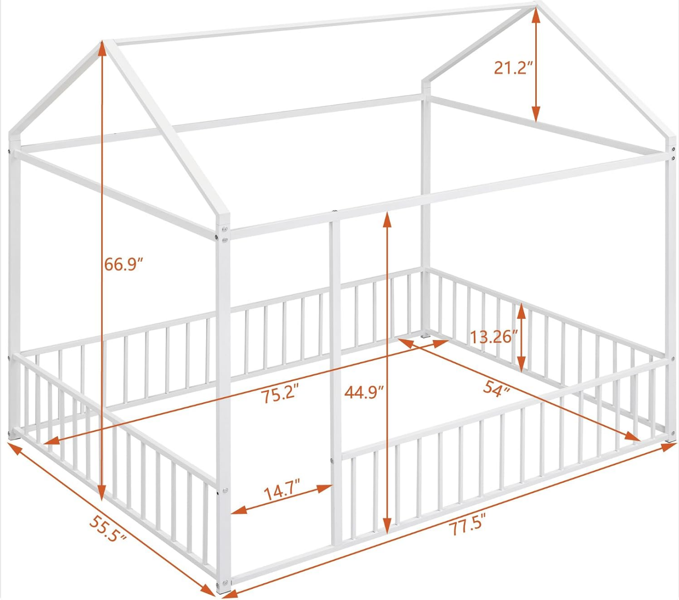
Image: Detailed dimensions of the Bellemave Full Floor Bed Frame, indicating overall length, width, and height.
