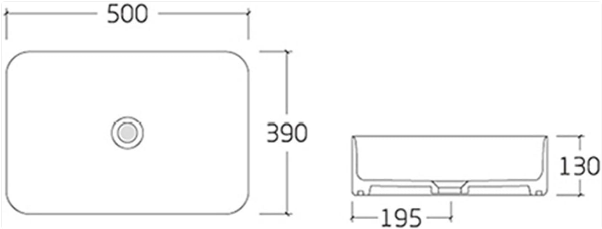
Figure 2: Technical drawing illustrating the dimensions of the JUNIKO II washbasin (Length 500mm, Depth 390mm, Height 130mm).
