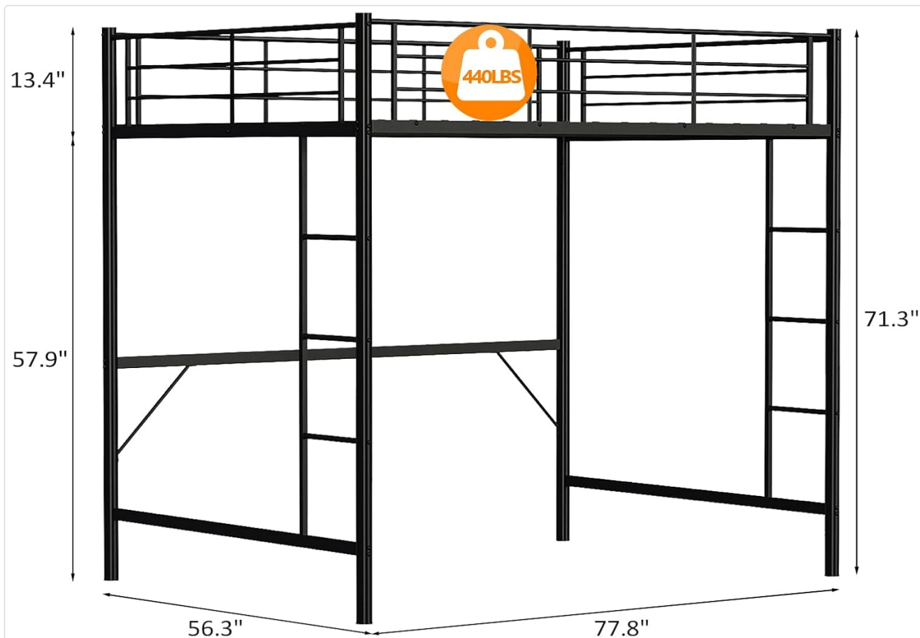
Figure 2: Product Dimensions and Key Features
